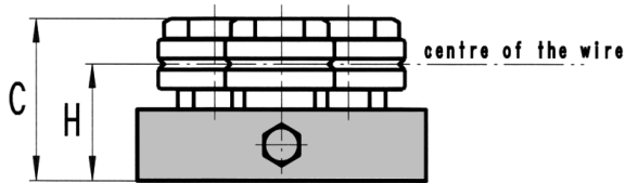
RB3 - Three Roll Unit
